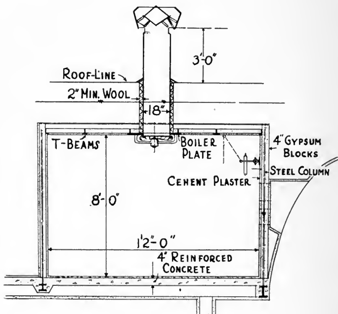
FIG. 3. Cross-section of projection room.
